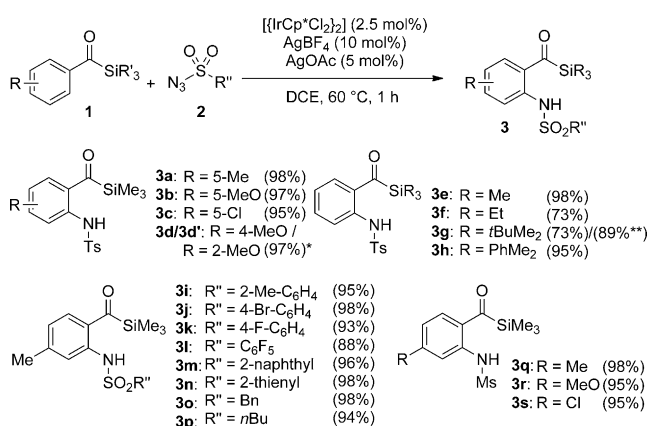
Scheme 2. Iridium-catalyzed ortho -amidation of aroylsilanes (*: obtained as a ca. 4:1 regioisomeric mixture; **: reaction time of 2 h). DCE = 1,2-dichloroethane, Ts = p -toluenesulfonyl.
